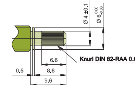
TYPE 0H - BRASS
