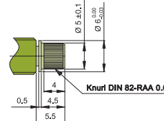
TYPE 44 - BRASS
