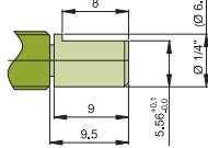
TYPE 13 - STAINLESS STEEL
