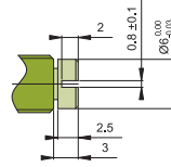
TYPE 02 - BRASS
