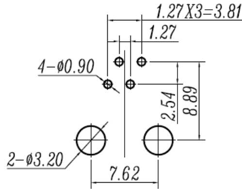
PC Board Layout Top View
