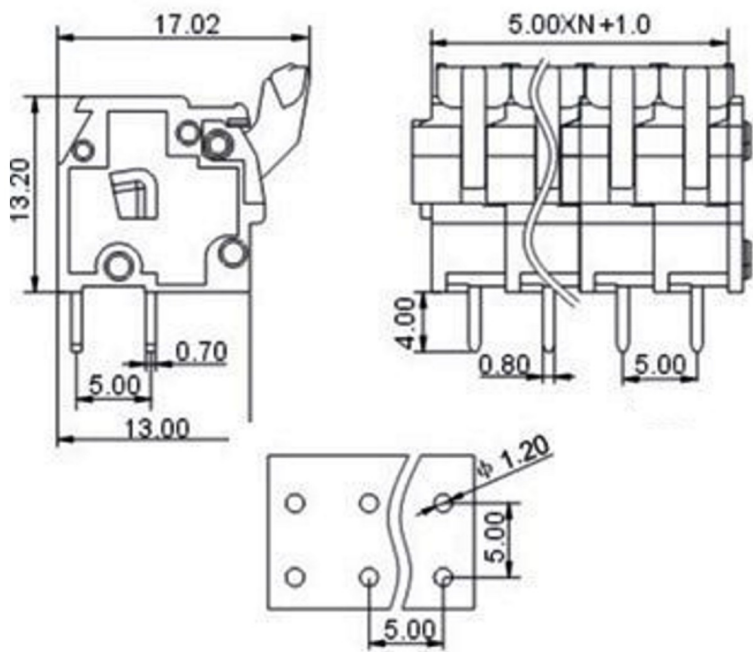
PCB LAYOUT
