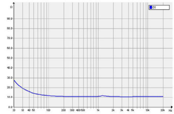
Impedance Curve
